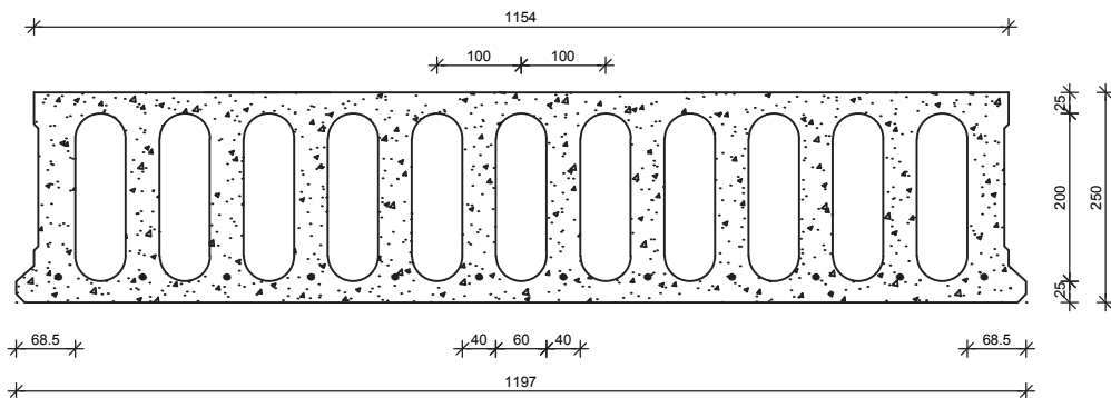
TOPFLOOR 250mm DEEP SLAB
