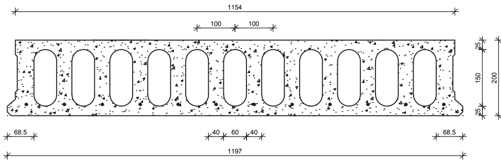
TOPFLOOR 200mm DEEP SLAB
