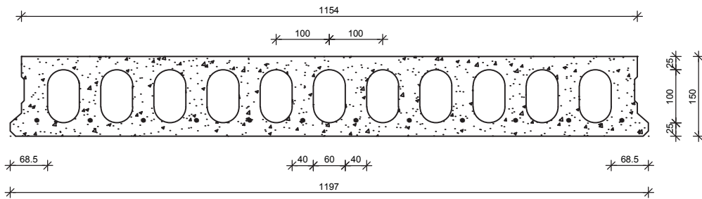
TOPFLOOR 150mm DEEP SLAB
